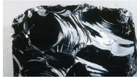
Obsidian Credit: ©Dr. Richard Busch, from the ESW Image Bank
